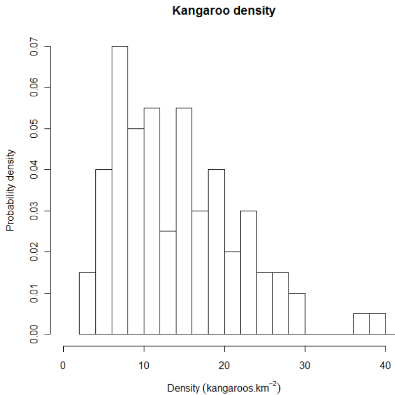
Figure 8: Histogram of a theoretical population of kangaroos.
