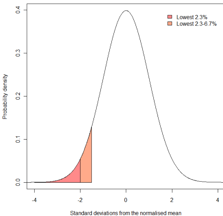
Figure 9: A theoretical distribution after z-score transformation.
